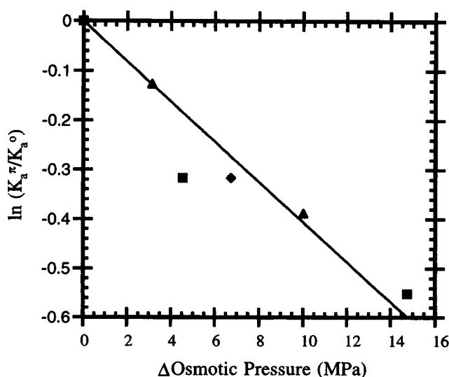
FIGURE 2 Normalized association constant obtained from equilibrium measurements by fluorescence polarization as a function of osmotic pressure for the three osmolytes glycerol (▲), ethylene glycol (■), and betaine (◆), fitted to \Delta \pi \Delta V_w = RT \ln(K_a^{\pi}/K_a^o) . Linear regression gives \sim 6.0 \pm 1.0 water molecules taken up on complex formation.
