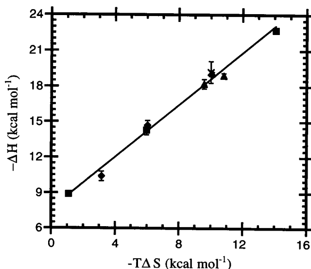
FIGURE 5 Enthalpy-entropy compensation plot (based on the data presented in Table 3) for the association of HyHEL-5 with BWQL in the presence of osmolytes (glycerol (▲), ethylene glycol (■), and betaine (◆)) or without osmolyte (×). The error in -T\Delta S is less than about \pm 0.3 kcal \text{mol}^{-1} .
