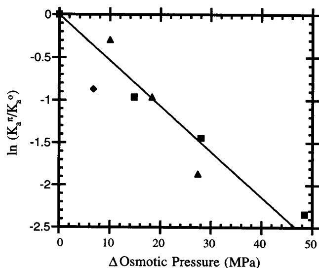
FIGURE 4 Normalized association constant obtained from equilibrium measurements by titration calorimetry as a function of osmotic pressure for the three osmolytes glycerol (▲), ethylene glycol (■), and betaine (◆), fitted to \Delta\pi\Delta V_w = RT \ln(K_a^pi/K_a^o) . The data point corresponding to 50% (w/w) betaine is not shown, because of nonavailability of osmotic pressure for betaine solution of this concentration. Linear regression gives \sim 8.0 \pm 1.0 molecules taken up on complex formation.
