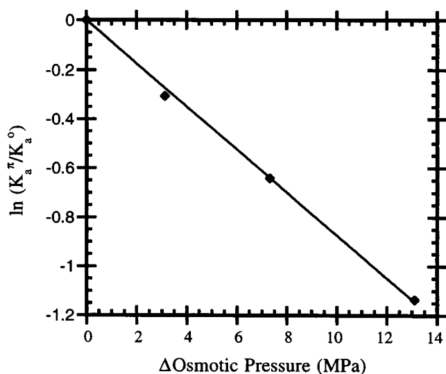
FIGURE 3 Normalized association constant calculated from kinetic measurements as a function of osmotic pressure for glycerol. Linear regression of the data gives \sim 12.0 \pm 3.0 water molecules taken up in the HyHEL-5/BWQL association.
